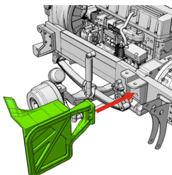
PE-part #33
